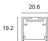
Profile section
