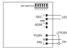
PUSH wiring diagram
